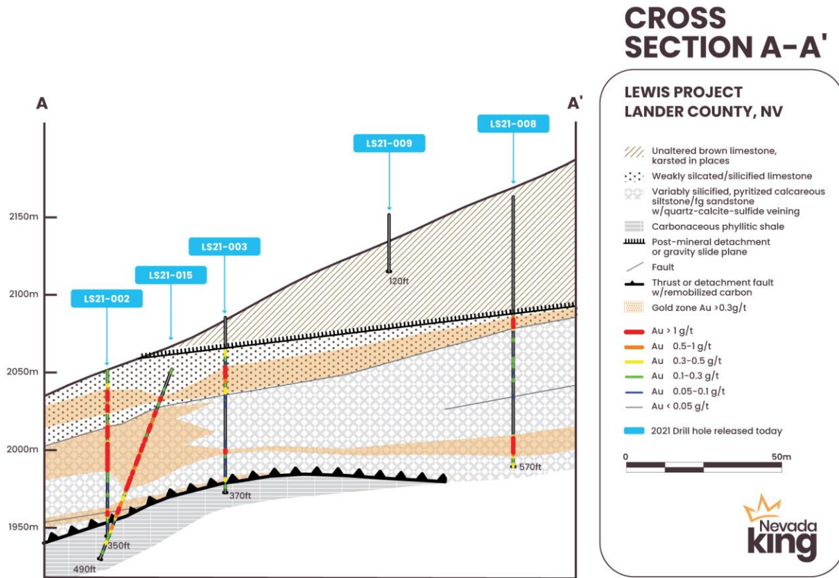
Figure 23. Drill section A-A' looking east at the Celestine O'Neal target area at the shallow dipping mineralized zone obscured by non-mineralized limestone emplaced along a landslide plane or detachment fault. LS21-008 hit 1.5 meters grading 15.73 g/t Au at 163-meter (535') depth.
