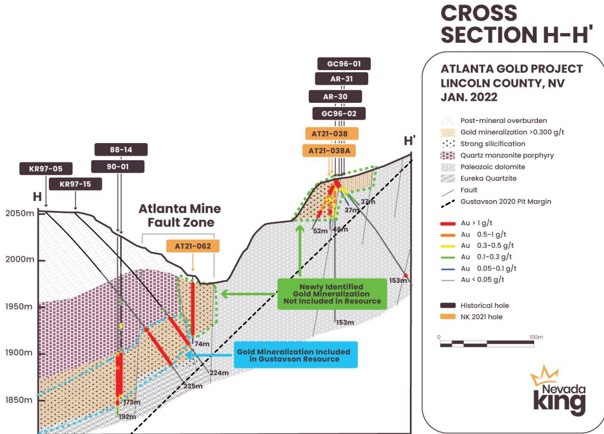
Figure 8. Cross section H-H' showing gold distribution in the Nevada King RC holes drilled across the center of the historical Atlanta open pit. Eastern margin of 2020 Gustavson gold resource model is located west and below intercept in AT21-062. Gold mineralization hit in AT21-062 extends the Gustavson resource model further eastward and up to the bottom of the pit.
