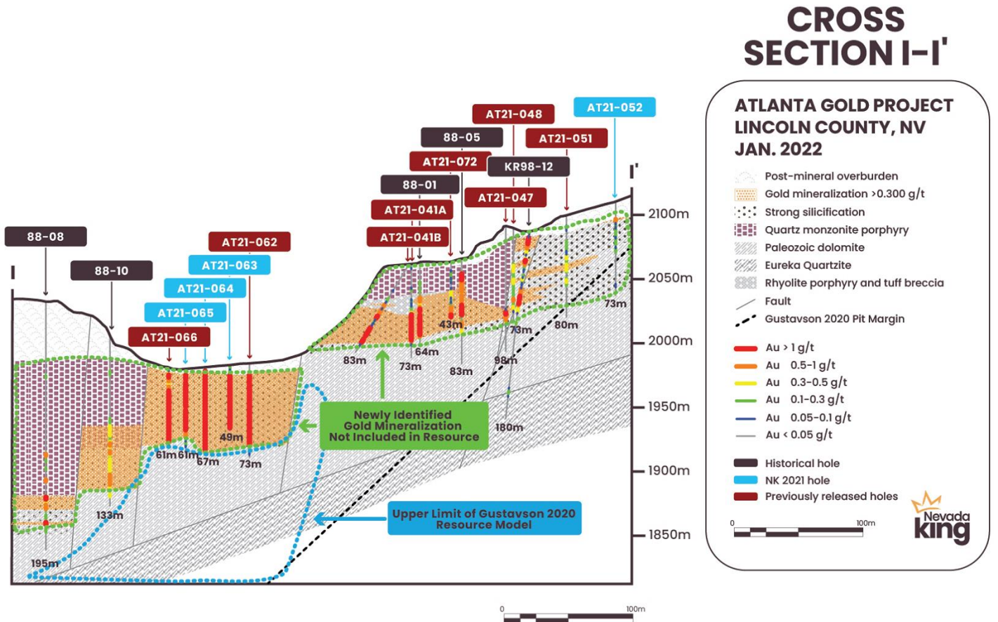
Figure 10. Cross section I-I' showing distribution of high-grade intercepts drilled from surface at the bottom of the historic pit in a fence of 5 RC drill holes from the Phase I 2021 drill campaign. Mineralization hit within AT21-066 – AT21-062 extends the upper limit of the Gustavson 2020 Resource Model up to the bottom of the existing pit.
