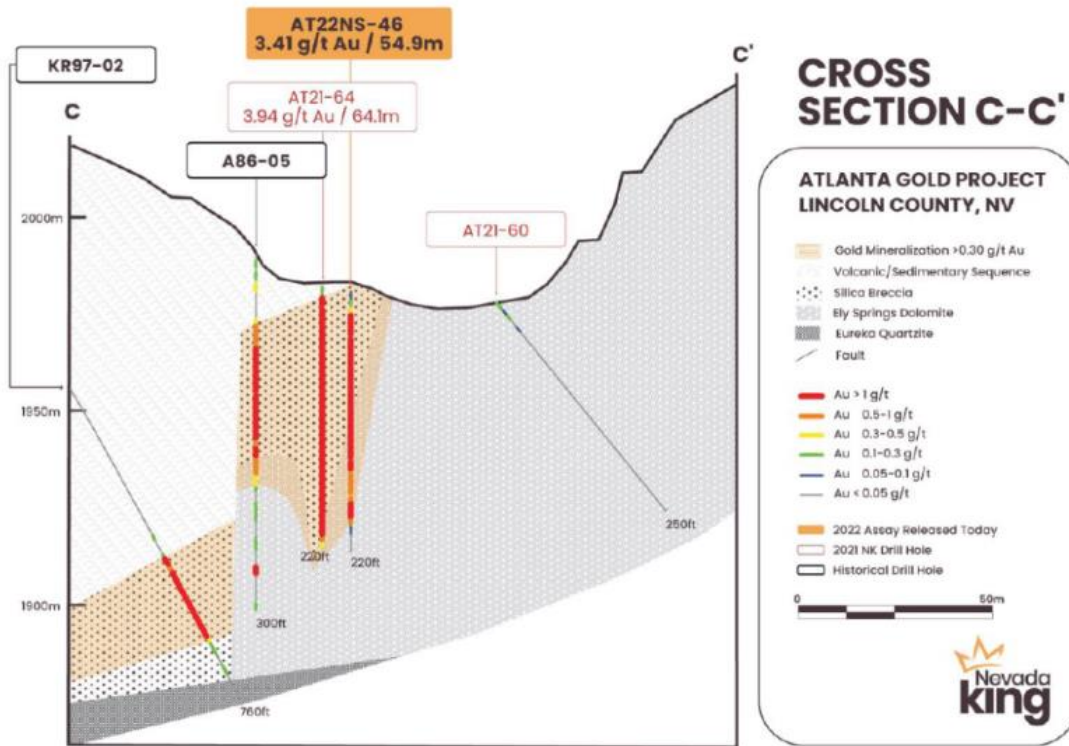
Figure 15. Cross section C-C' looking north across the center of the historical Atlanta pit illustrating normal fault displacement on the steeply dipping Atlanta Mine Fault and progressive down-drop across parallel faults to the west. The Eureka Quartzite is shown in fault contact with the silica breccia and dolomite units and appears to cut off the Atlanta Fault at depth, but this interpretation is based on historical drill hole, and in other sections the Atlanta Fault clearly displaces the quartzite contact.
