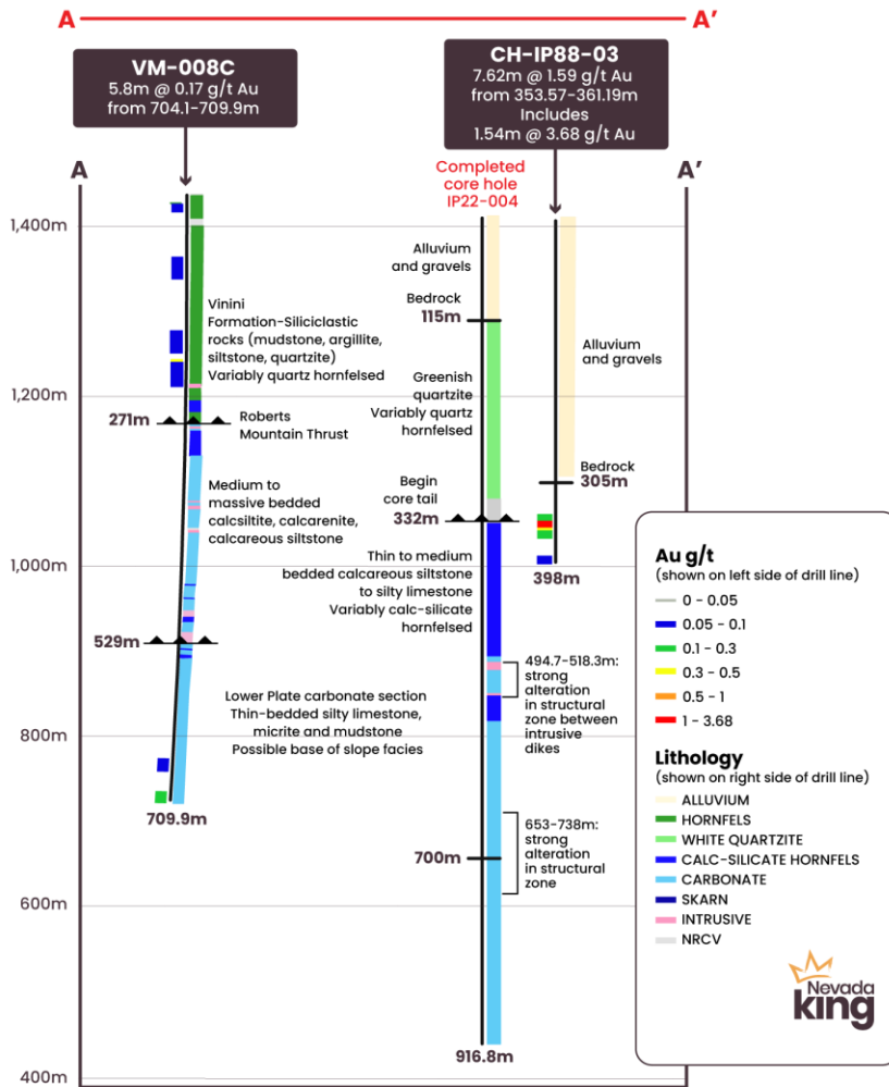
Figure 5. Cross Section A-A' across RFZ target area from 2019 Nevada King core hole VM-008C to 1988 Chevron RC hole CH-IP88-03, showing location of completed drill hole IP22-004.
