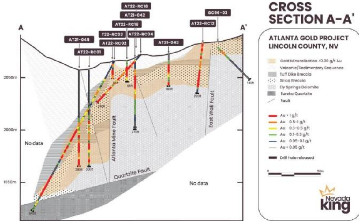
Figure 12. Section A-A' across the southern end of the historical Atlanta pit showing the “roll-over” in dip of the mineralized zone from horizontal on the east to 45 degrees on the west with the intersection of the mineralization by AT22-RC02 and AT22RC-12. Note the close relationship between felsic tuff dike breccia bodes and Au mineralization.
