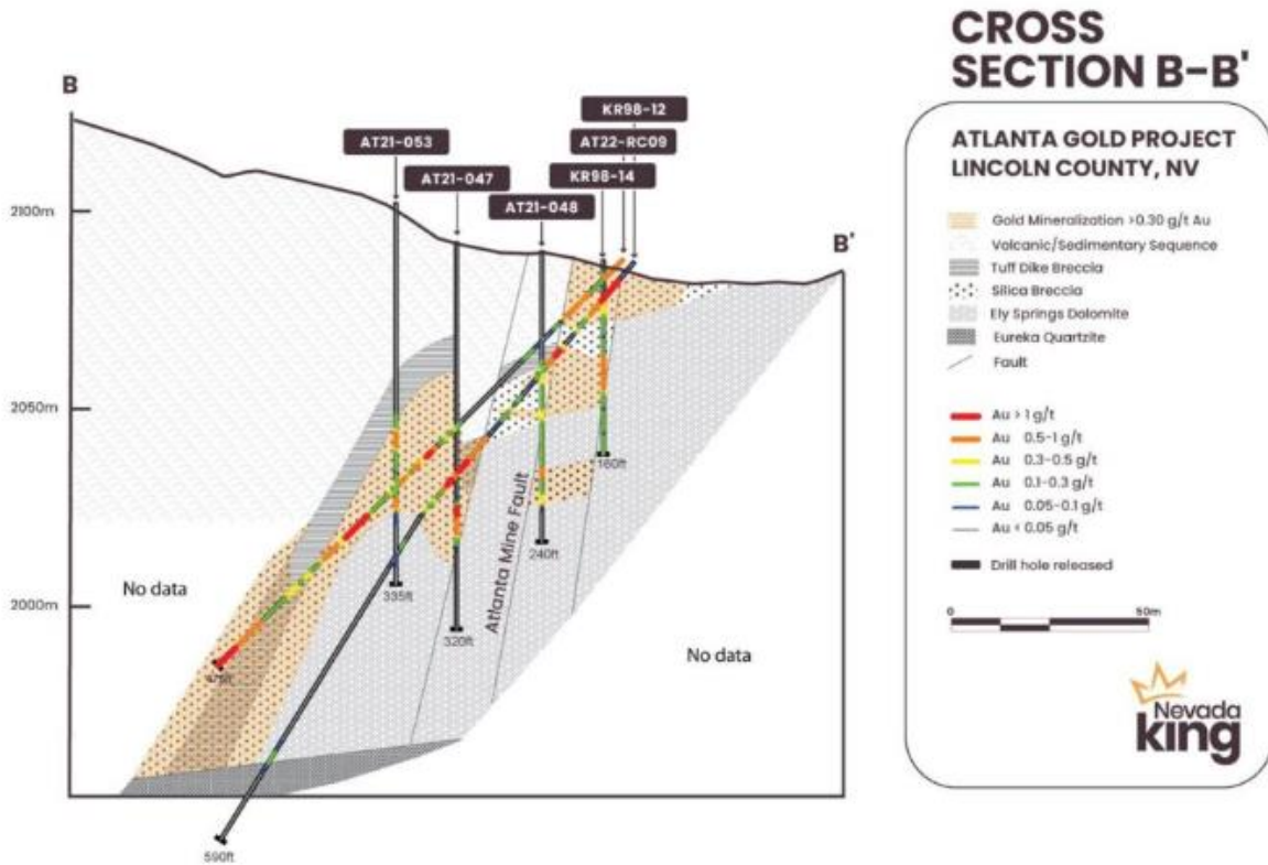
Figure 13. Section B-B' across the southern extension of the Atlanta Mine Fault Zone 150 meters south of the historical Atlanta pit, showing same dip roll-over in the mineralized zone and same Au-tuff dike breccia association as seen in Figure 12 to the north. More drilling is planned west of AT21-053 to follow-up the intercept in AT22-RC09.
