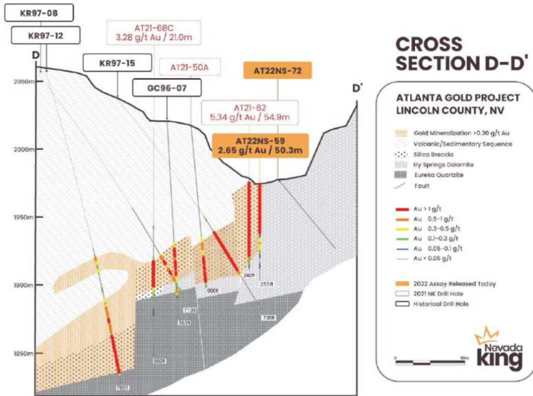
Figure 16. Cross section D-D' looking north across the south-central part of the historical Atlanta pit showing progressive down-drop of the mineralized silica breccia zone and the basal quartzite contact along a series of parallel faults comprising the Atlanta Mine Fault Zone. Note the start of gold mineralization in the volcanic/sedimentary package above the silica breccia horizon at the left side of the section.
