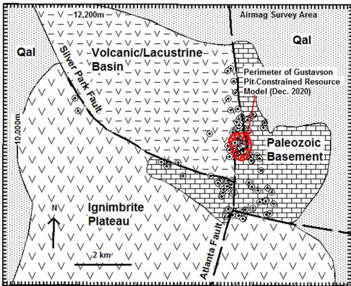
Figure 20. Generalized geology of the Atlanta district. Historical drill holes shown by circles. Atlanta open pit is located in the center of the 2020 Gustavson pit-constrained resource zone.
