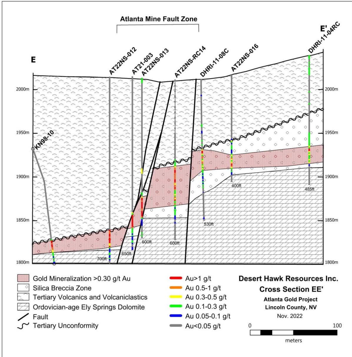
Figure 18. Cross section E-E' looking north across the northern extension of the AMFZ about 500 meters north of the historical Atlanta pit. Mineralization hit in historical hole 170 meters west of section and remains open to the west, while mineralization remains open east of DHRI-11-04RC. Westward normal fault displacement on the mineralized horizon across the steeply-dipping Atlanta Mine Fault is evident.
