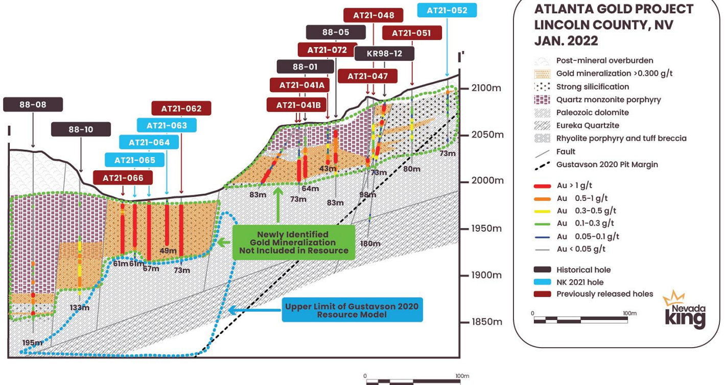
Figure 16. Cross section I-I' showing distribution of high-grade intercepts drilled from surface at the bottom of the historic pit in a fence of 5 RC drill holes from the Phase I 2021 drill campaign. Mineralization hit within AT21-066 – AT21-062 extends the upper limit of the Gustavson 2020 Resource Model up to the bottom of the existing pit.
