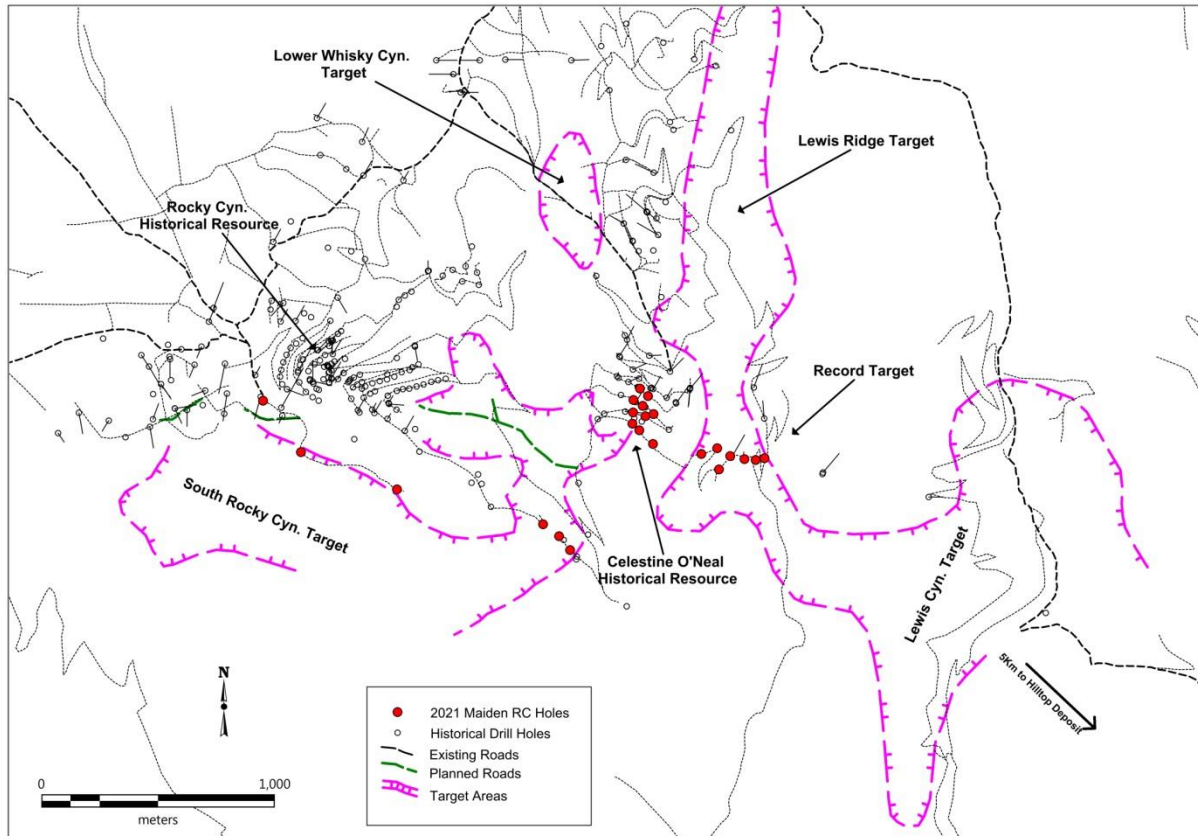
Figure 13. Location of proposed 2021 RC drill holes (red dots) relative to major exploration targets and existing roads (black dashed and dotted lines). Targets as denoted by the purple hatched target areas are defined by vectors derived from historical drill results together with surface sample results. Historical drill holes shown by black circles.
